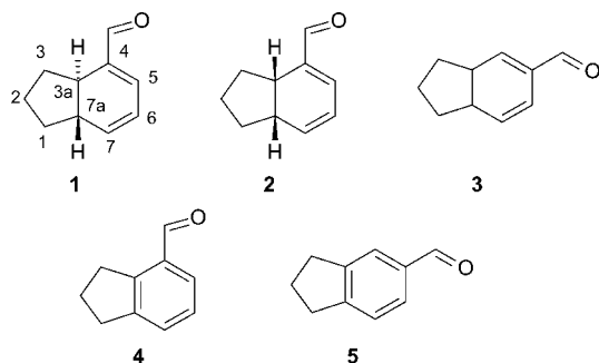
Figure 2. Structures of ( \pm )- cis/trans -2,3,3a,7a-tetrahydro-1H-indene-4-carbaldehyde 1 and 2 and related structures 3–5 .
